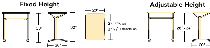
TD2027YADJBBM Adjustable-height desk with plastic book box. Work surface is 20" x 27" FRW hard plastic.
